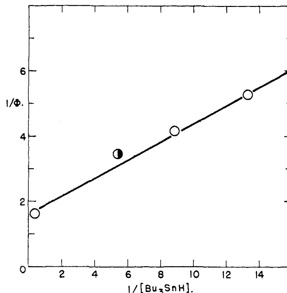
Fig. 3.—Photoreduction of 2-acetonaphthone by tri- n -butylstannane; ● is average of three determinations.
