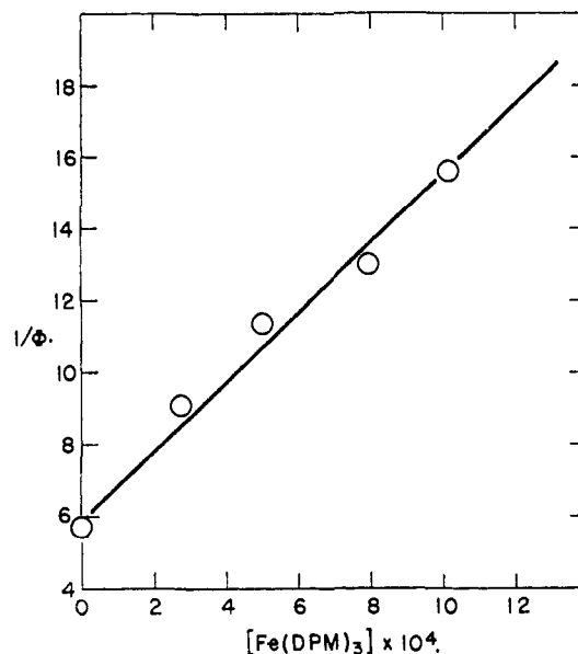
Fig. 2.—Quenching of the reduction of 1-naphthaldehyde by ferric dipivaloylmethide.
